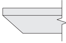
Reverse Bevel (E1) Veneer Band on Stained MDF
