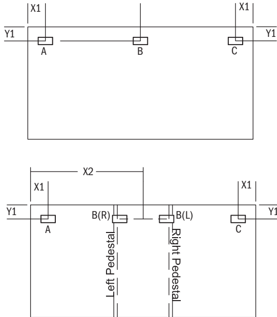
Diagram: G4 Applies to all bridge or return tops. Grommets cannot be placed over the top of a pedestals.
