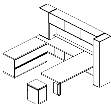
U-Group layout made up of built up, free standing casegood components, End Panel Desk, Full Height Access, Panel-Support Overhead, Tower, Wardrobe and Two-High Lateral
