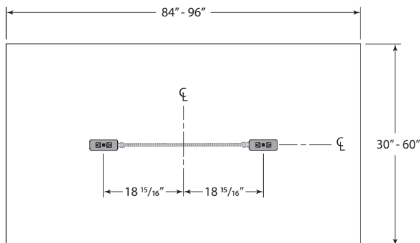
CT2 - Dual Power Top of Surface
